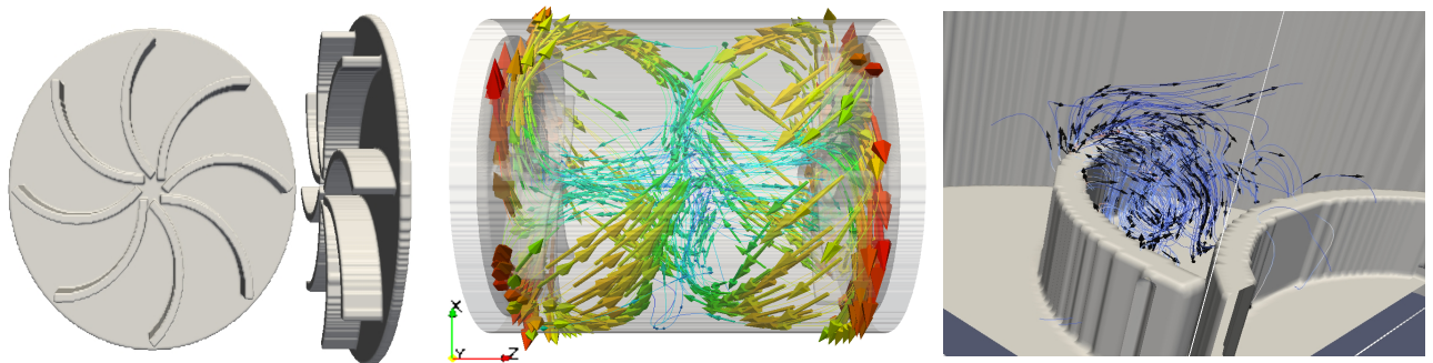
Figure 1: (left) Visualisation of the propeller built by penalisation leading to a Von Kàrmàn flow. (centre) Visualisation of the temporal mean flow. (right) Visualisation of the vortex produce by the propeller inside the rotation frame.
